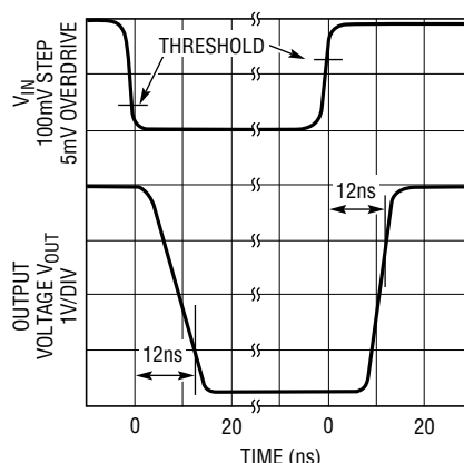
Comparator Response Time
